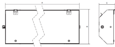
PITBUL-Ex, 4x58W, IP65
