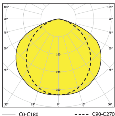
SALUKA-N-LED-236, IP66
